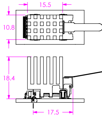
-2 PIN-FIN HEAT SINK
