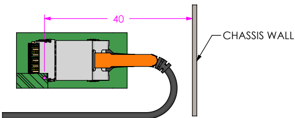
-7 FIBER TYPE RECOMMENDED CABLE ESCAPE CLEARANCE
