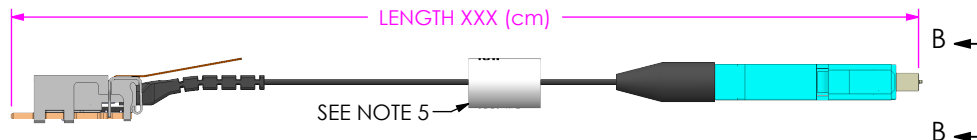
PART NUMBER ECUO-B04-XX-XXX-0-1-1-5-07 SHOWN
