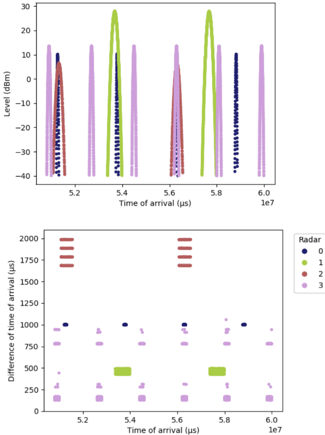
Fig. 7. Final grouping of clusters according to HAC results with POT measurements. We used the dendrogram to group clusters and obtained this representation. The colors represent the final clusters and the 4 emitters present. The DTOA was calculated from the pulses of each emitter.
