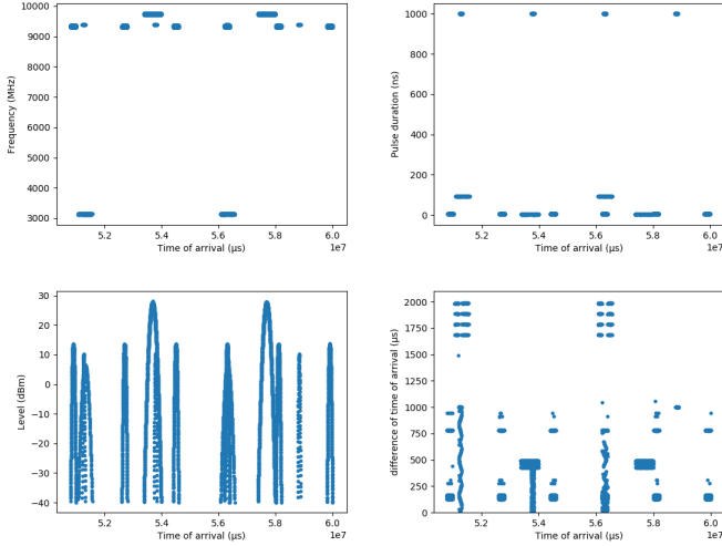
Fig. 3. The figure represents a signal without any indication of the number of transmitters present. The signal is represented using its primary parameters (F, PW, G, DTOA and TOA). The signal has not been represented entirely, a zoom has been applied to facilitate its visualization. The DTOA has been calculated on the whole signal.
