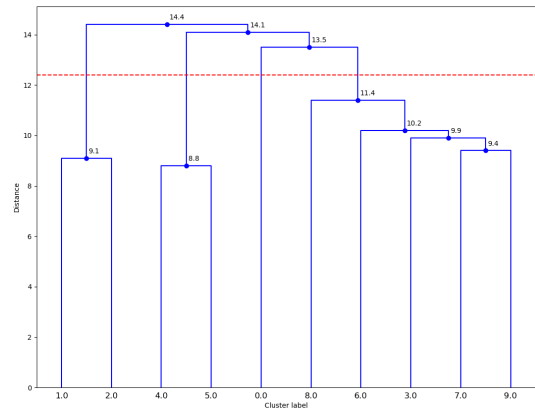
Fig. 6. Hierarchical agglomerative clustering results in logarithmic form with Optimal transport measures. We constructed decision rules from the optimal transport values using several metrics to determine where to cut the dendrogram. The red line indicates where to cut the dendrogram. Here the metrics tell us that our signal contains pulses from 4 different transmitters.
