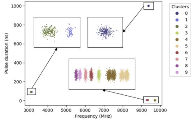
Fig. 5. Results of HDBSCAN clustering in the F-PW plan. A zoom has been applied in the F-PW plane. Colors represent the 10 different clusters returned by the algorithm. Clusters are distributed along the lobes in the G-TOA plane.
