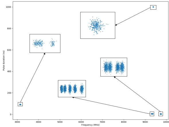
Fig. 4. Zoom on the F-PW plane of the previous signal.
