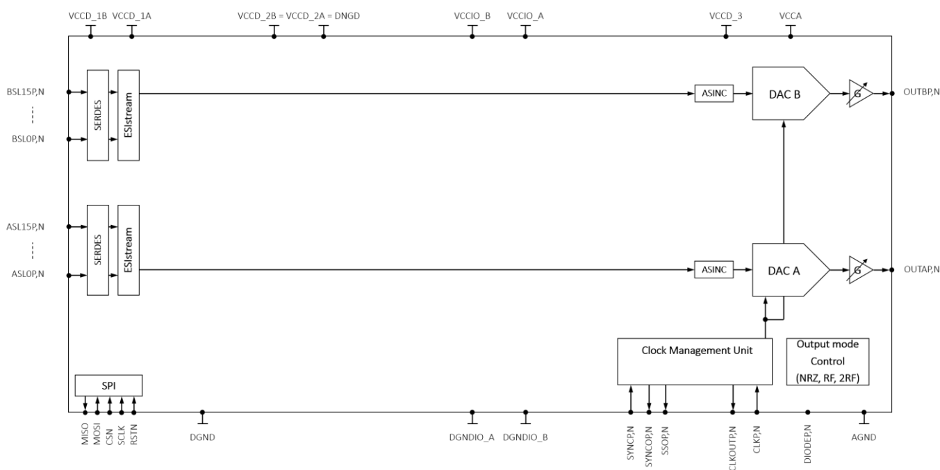
Figure 2: Simplified Block Diagram using Real data
