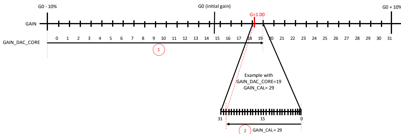
Figure 15: Gain adjustment trough x\_GAIN\_CAL & GAIN\_DAC\_CORE
