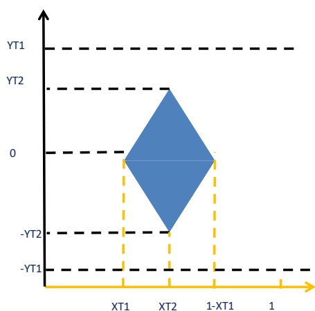
Figure 4 - Serial link eye diagram
