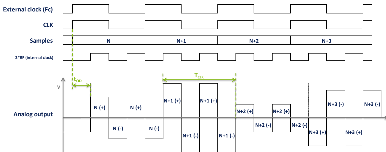
Figure 19 – 2RF mode timing diagram
