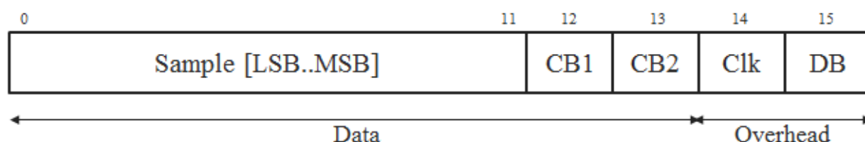
Figure 14: ESistream frame with EV12DD700
