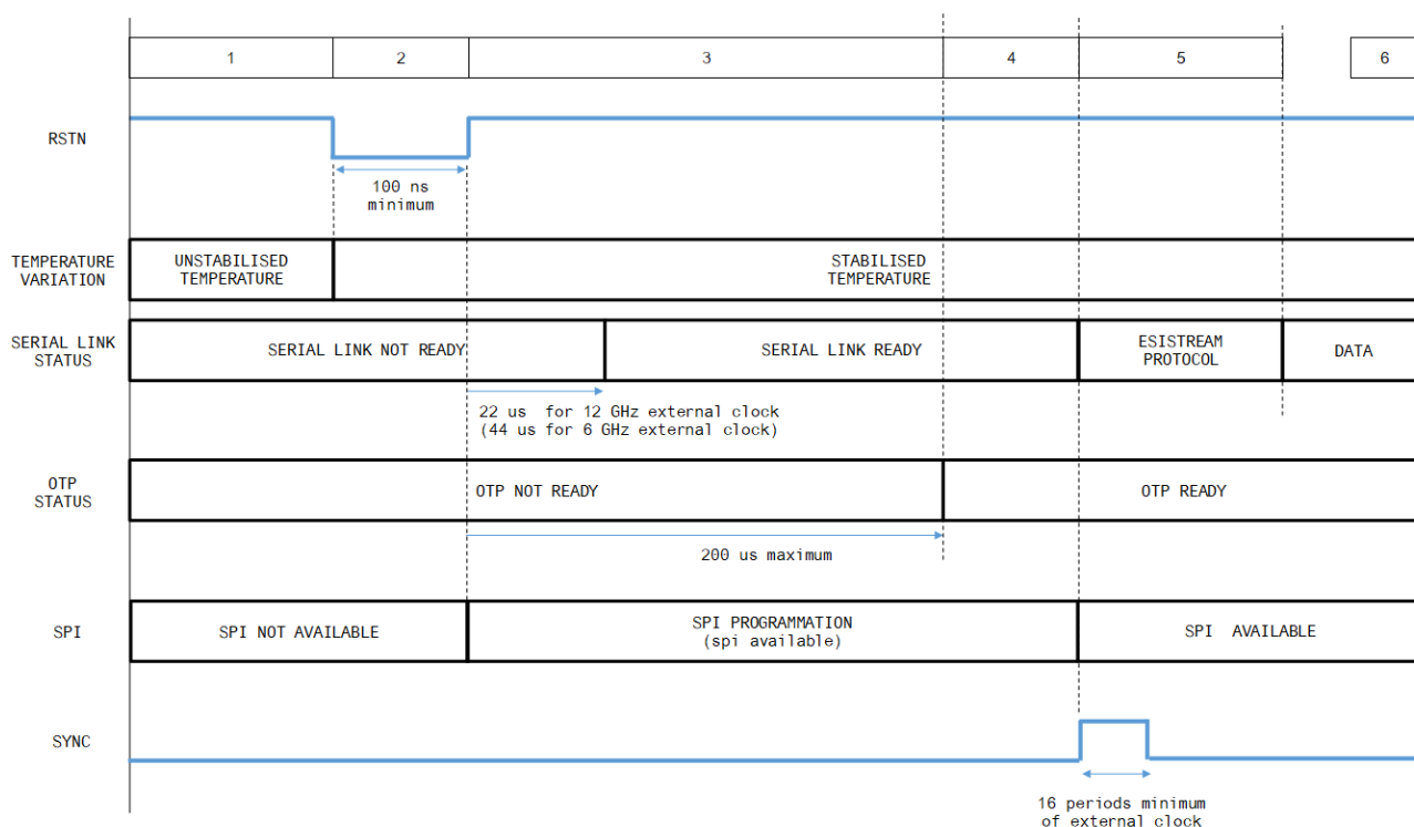
Figure 54: Start-up sequence
