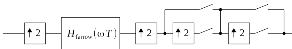
Figure 22 – Signal path before mixer
