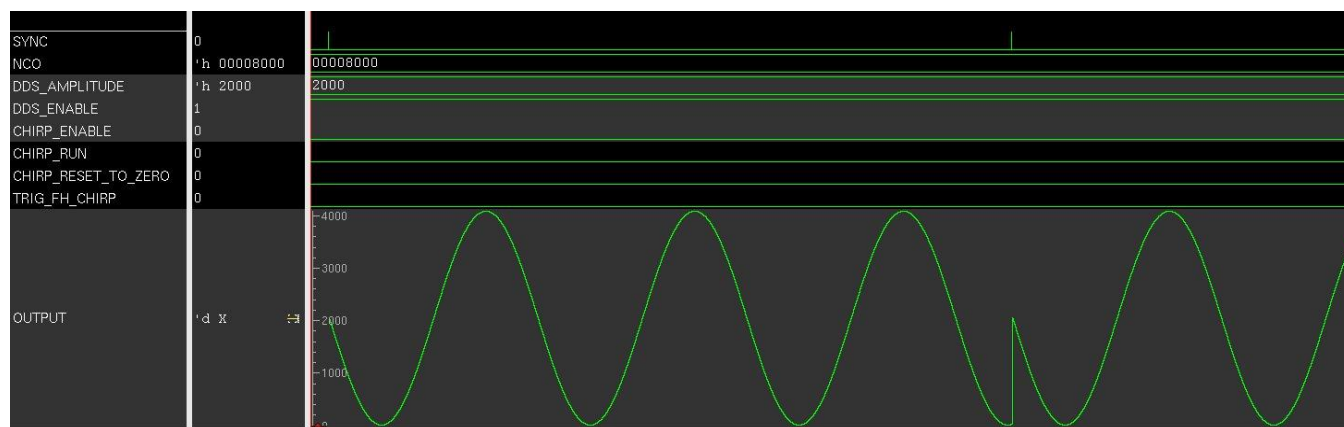
Figure 36 – DDS mode
