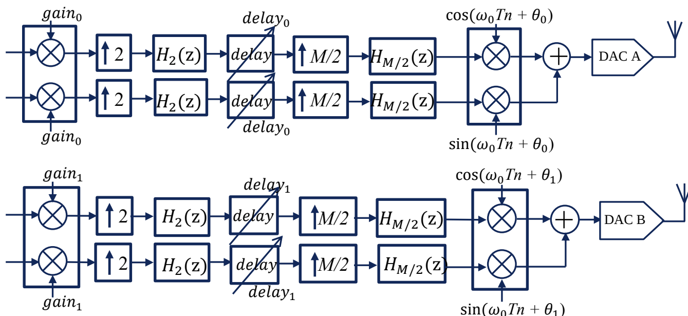
Figure 33 – Beam-forming (Digital Butler Matrix) principle
