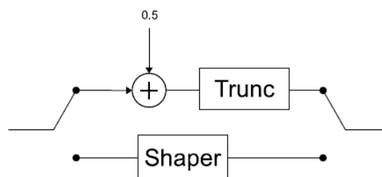
Figure 30 – NCO Truncation selection
