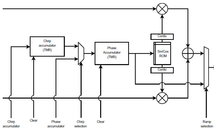
Figure 38 – Complex mixer configuration for Chirp function
