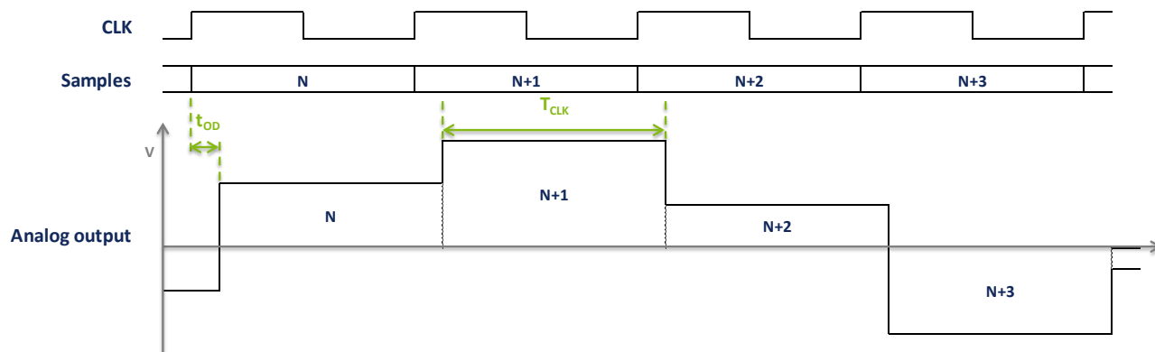
Figure 17 – NRZ mode timing diagram
