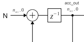
Figure 26 – Phase accumulator
